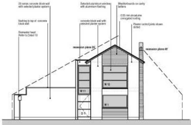
EAST ELEVATION
