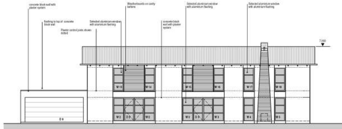
NORTH ELEVATION
