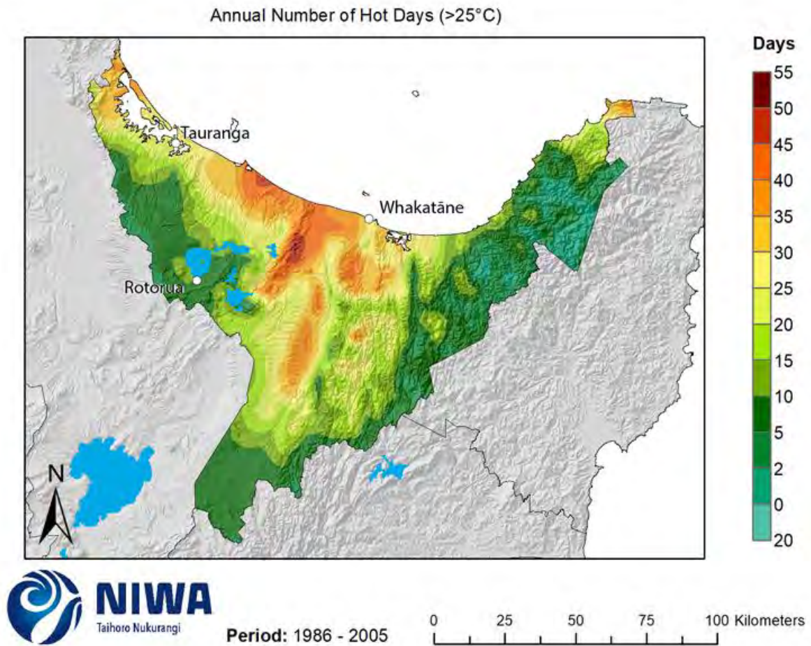
Figure 3-21: Modelled annual number of hot days (days with maximum temperature >25°C), average over 1986-2005. Results are based on dynamical downscaled projections using NIWA's Regional Climate Model. Resolution of projection is 5km x 5km.
