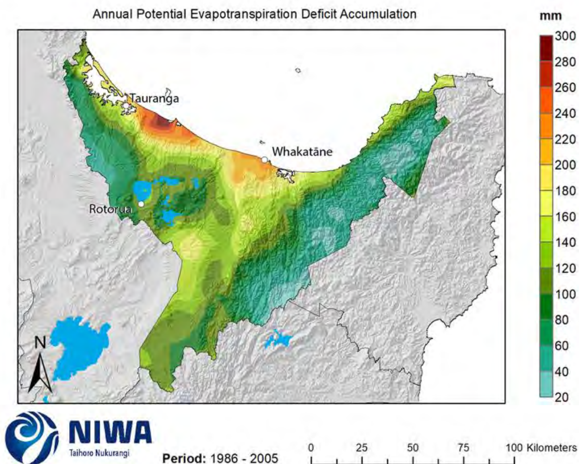
Figure 4-27: Modelled annual potential evapotranspiration deficit accumulation (mm), average over 1986-2005. Results are based on dynamical downscaled projections using NIWA's Regional Climate Model. Resolution of projection is 5km x 5km.
