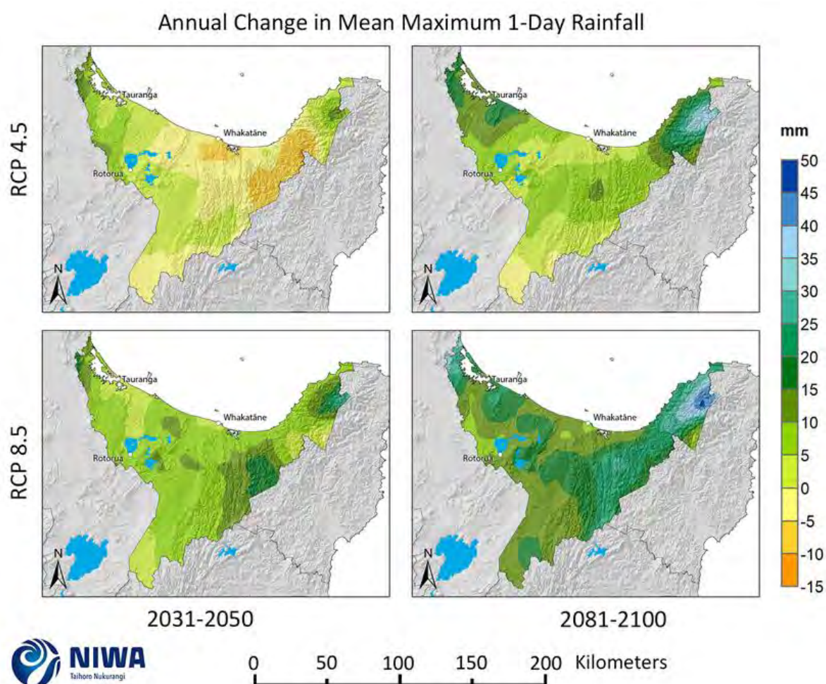
Figure 4-19: Projected annual mean maximum 1-day rainfall (Rx1day) changes for RCP4.5 and RCP8.5, by 2040 and 2090. Relative to 1986-2005 average, based on the average of six global climate models. Results are based on dynamical downscaled projections using NIWA's Regional Climate Model. Resolution of projection is 5km x 5km.
