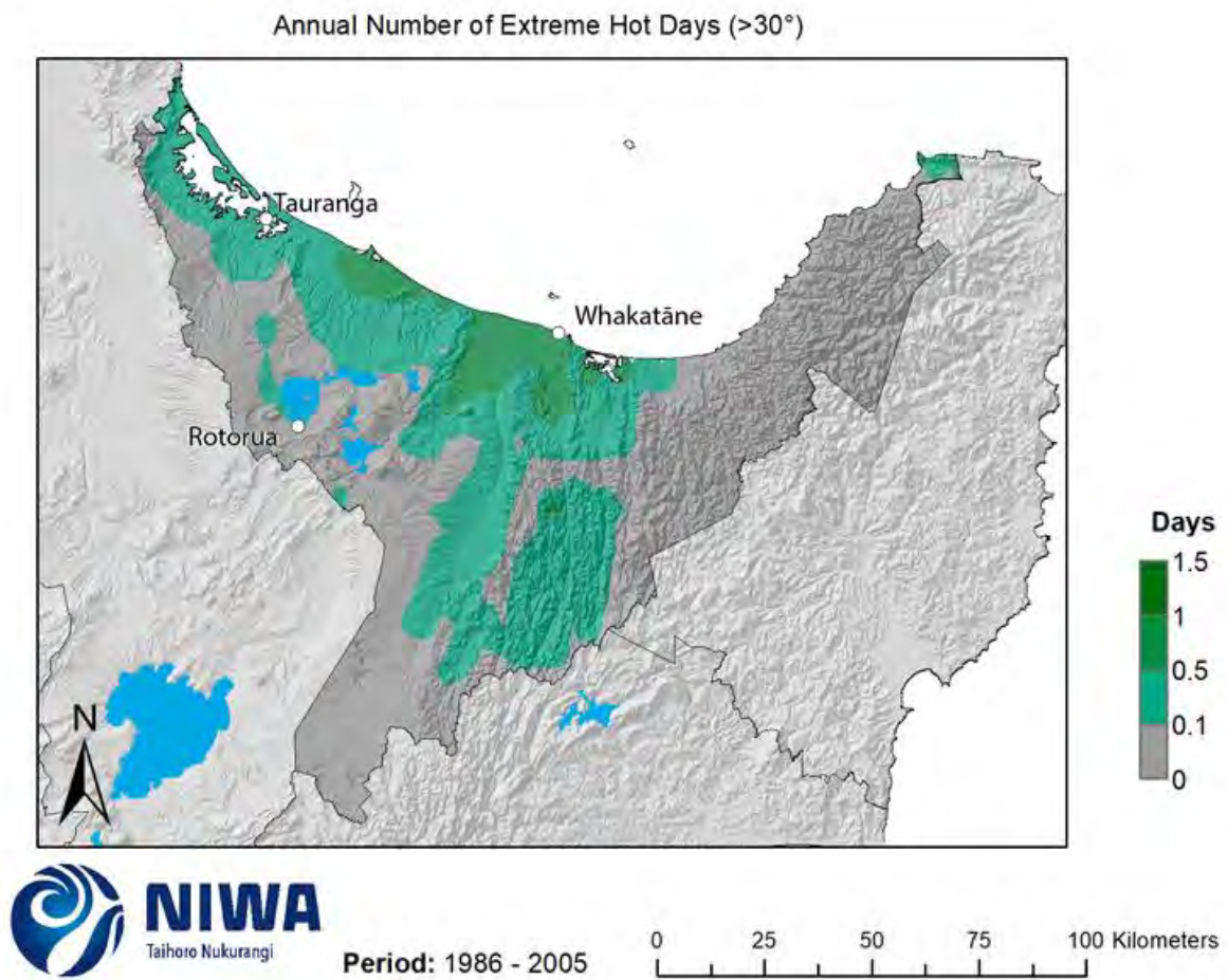
Figure 3-24: Modelled annual number of extreme hot days (days with maximum temperature >30°C), average over 1986-2005. Results are based on dynamical downscaled projections using NIWA's Regional Climate Model. Resolution of projection is 5km x 5km.
