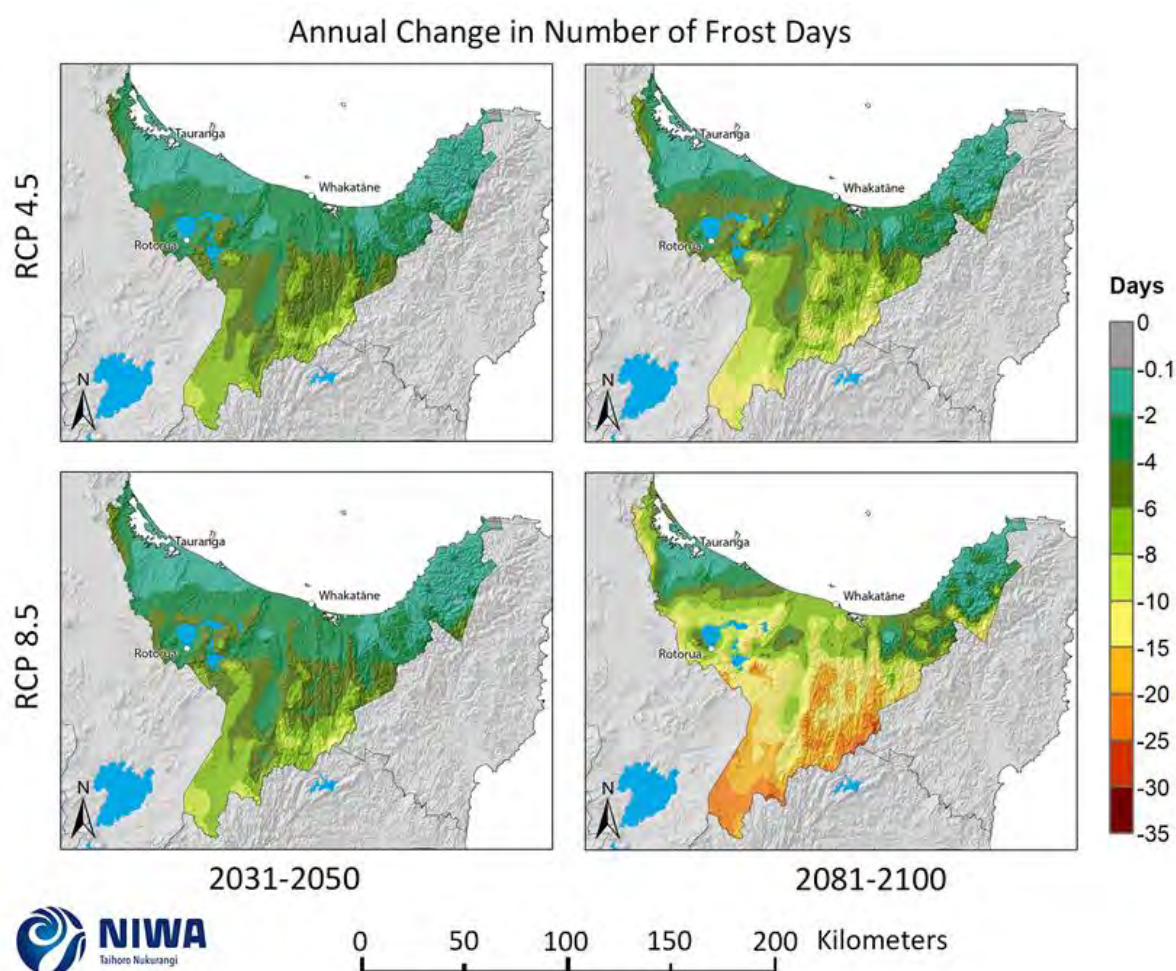
Figure 3-29: Projected annual frost day (minimum temperature <0°C) changes for RCP4.5 and RCP8.5, by 2040 and 2090. Relative to 1986-2005 average, based on the average of six global climate models. Results are based on dynamical downscaled projections using NIWA's Regional Climate Model. Resolution of projection is 5km x 5km.
