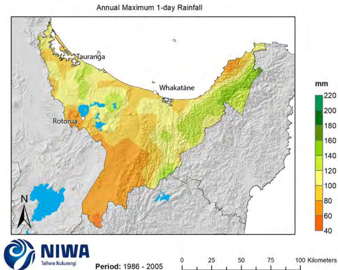
Figure 4-18: Modelled annual maximum daily rainfall (Rx1day), average over 1986-2005. Results are based on dynamical downscaled projections using NIWA's Regional Climate Model. Resolution of projection is 5km x 5km.
