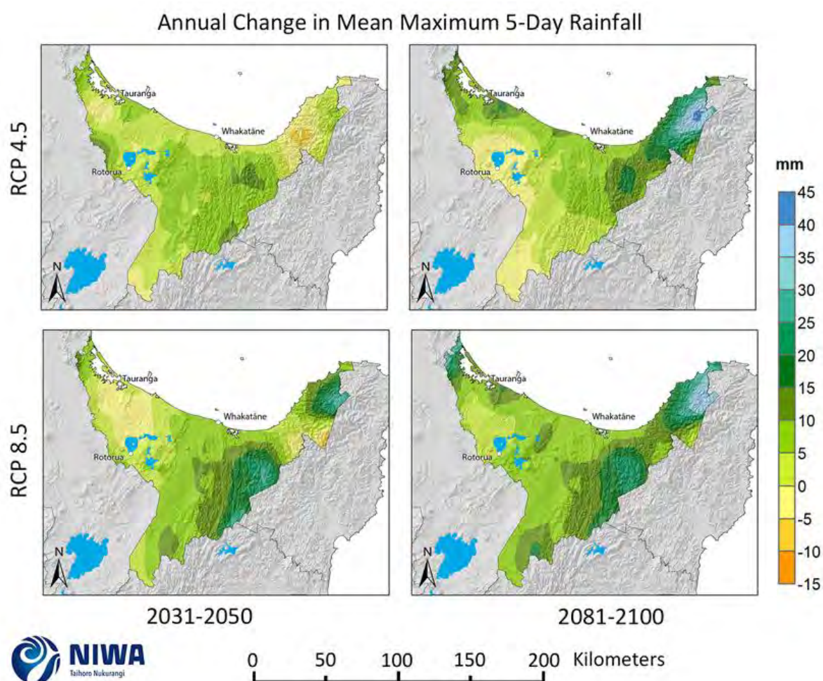
Figure 4-21: Projected annual mean maximum 5-day rainfall (Rx5day) changes for RCP4.5 and RCP8.5, by 2040 and 2090. Relative to 1986-2005 average, based on the average of six global climate models. Results are based on dynamical downscaled projections using NIWA's Regional Climate Model. Resolution of projection is 5km x 5km.
