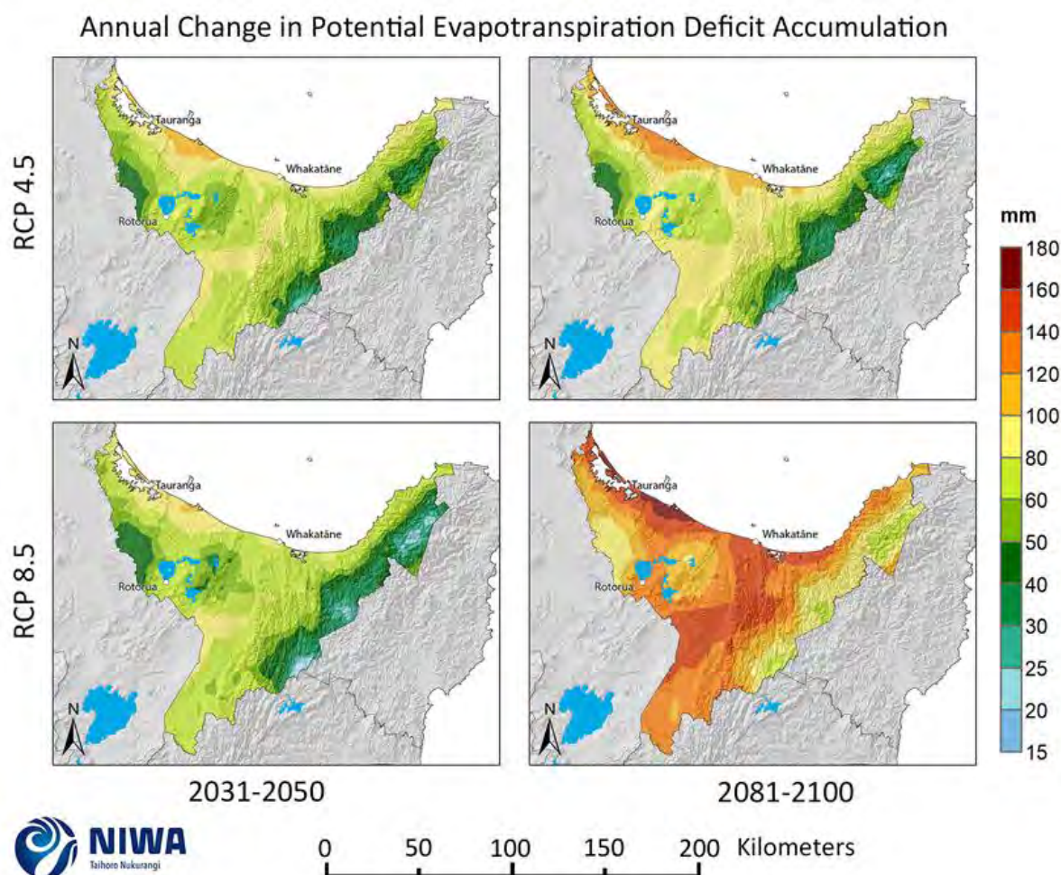
Figure 4-28: Projected annual potential evapotranspiration deficit (PED) accumulation changes for RCP4.5 and RCP8.5, by 2040 and 2090. Relative to 1986-2005 average, based on the average of six global climate models. Results are based on dynamical downscaled projections using NIWA's Regional Climate Model. Resolution of projection is 5km x 5km.
