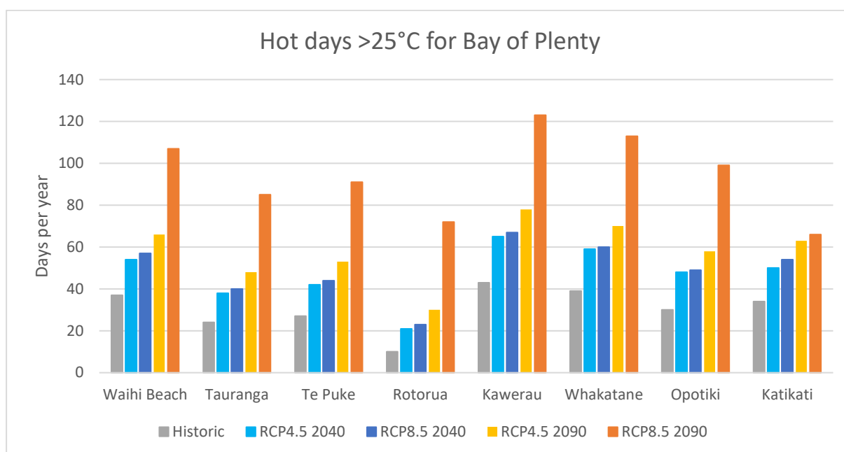
Figure 3-23: Historic and future projected numbers of hot days for locations in the Bay of Plenty.
