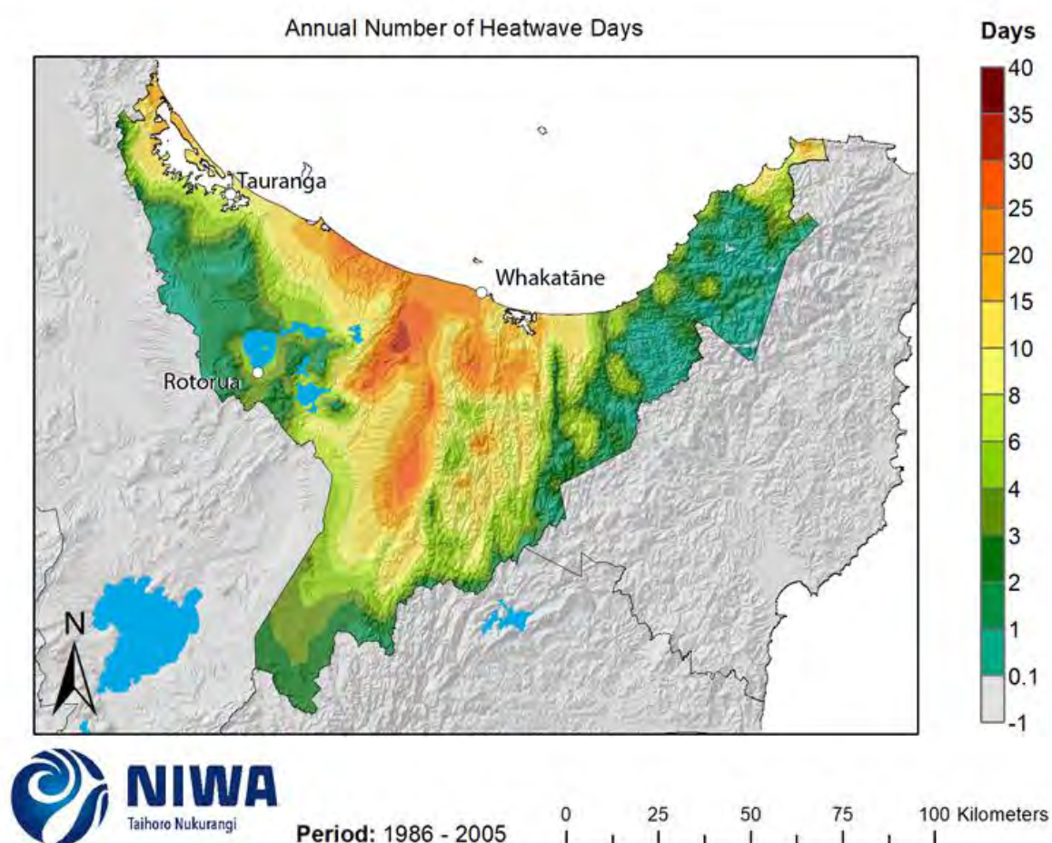
Figure 3-26: Modelled annual number of heatwave days (≥ three consecutive days with maximum temperatures > 25°C), average over 1986-2005. Results are based on dynamical downscaled projections using NIWA's Regional Climate Model. Resolution of projection is 5km x 5km.
